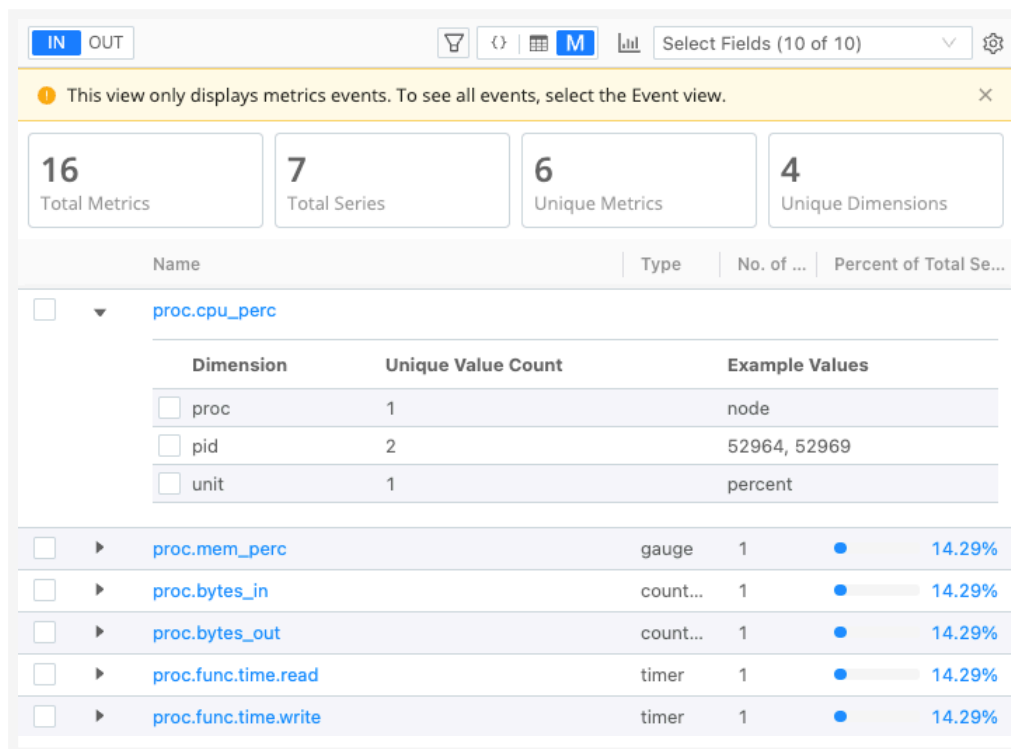
Example Metrics View
