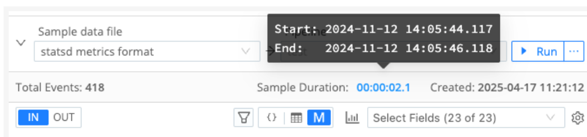
Hover over the Sample Duration to view start and end times
