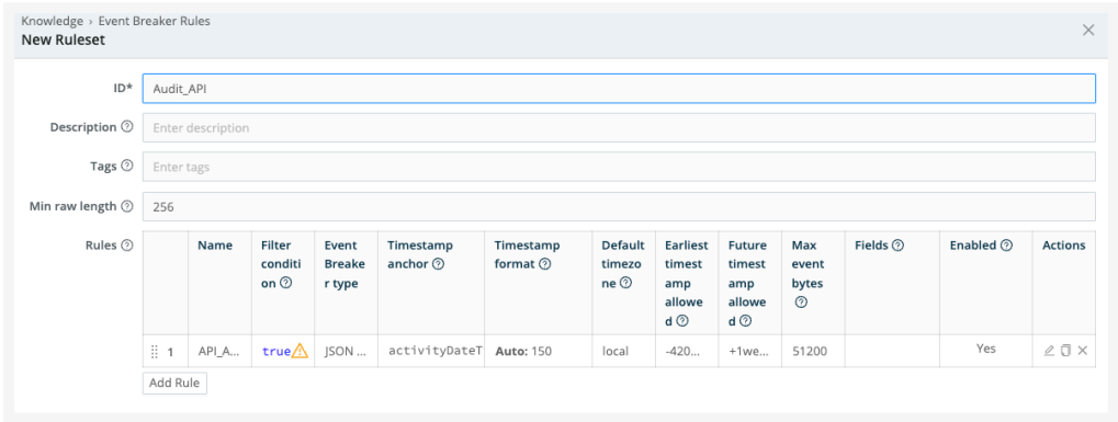
Creating an Event Breaker Ruleset for Audit Logs data
