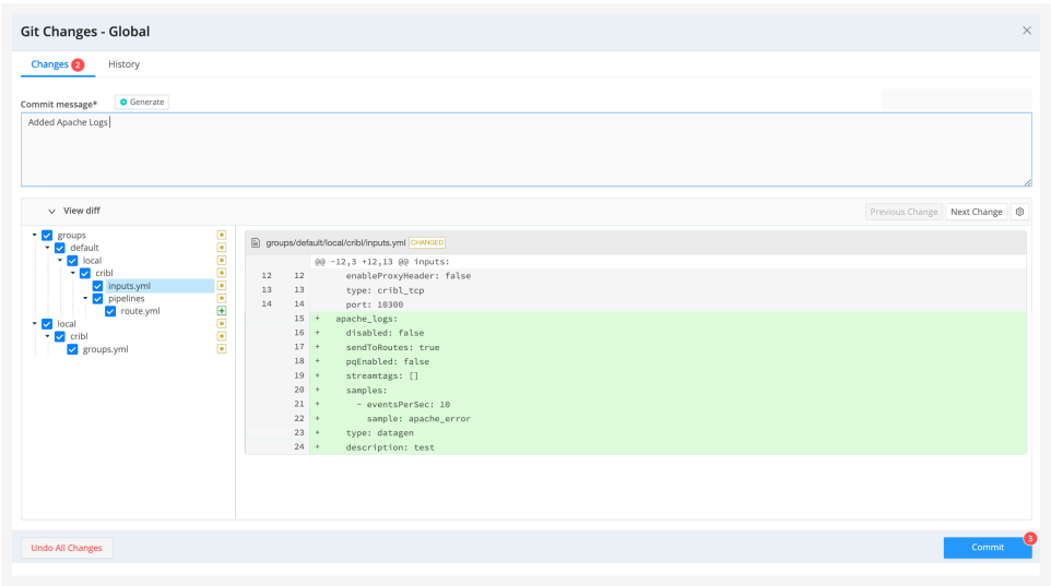
Review the pending commit
