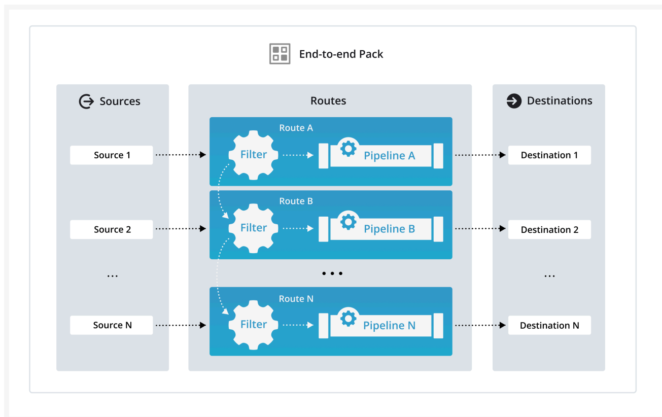
Packs can contain end-to-end data flow components
