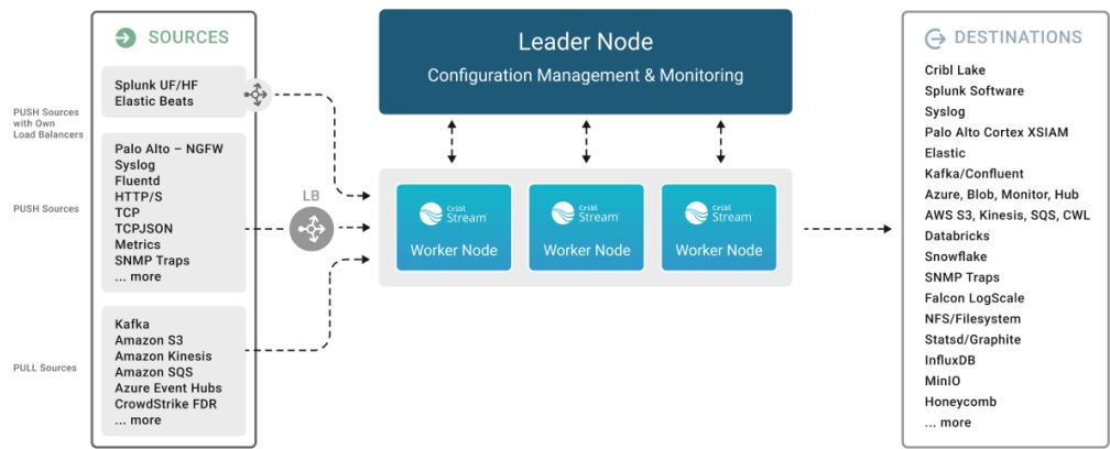
Push and Pull Sources
