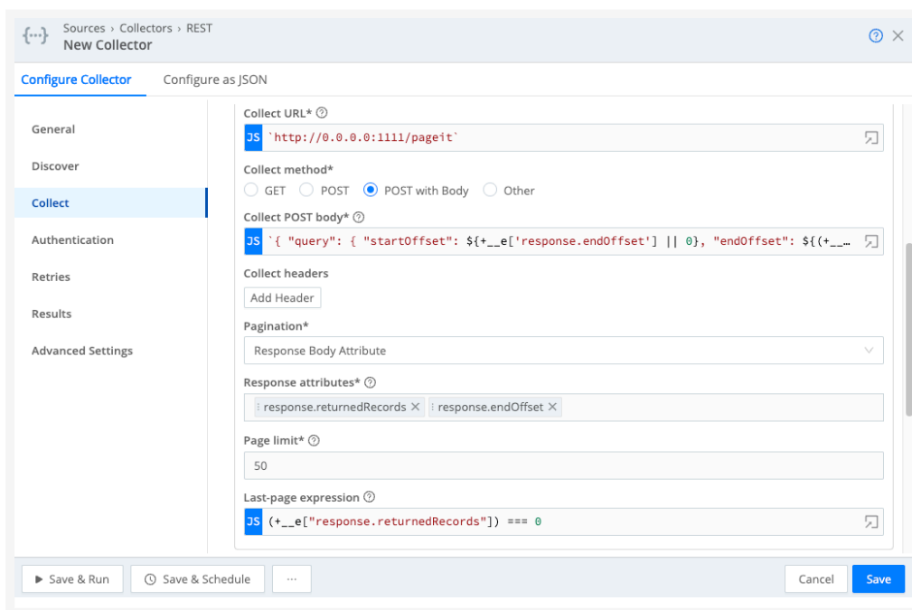
Collect POST body and Last-page expression
