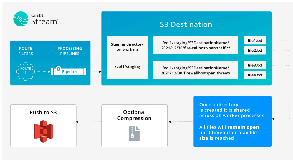
Write to object storage - example
