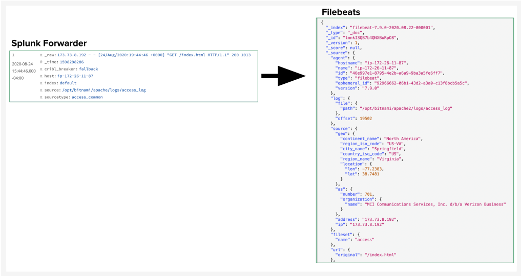
Transforming to Elastic Common Schema
