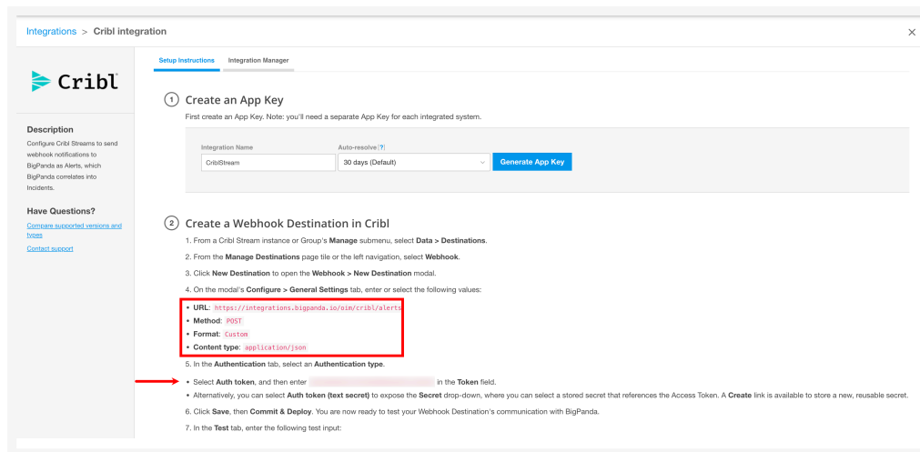
The Cribl Integration page
