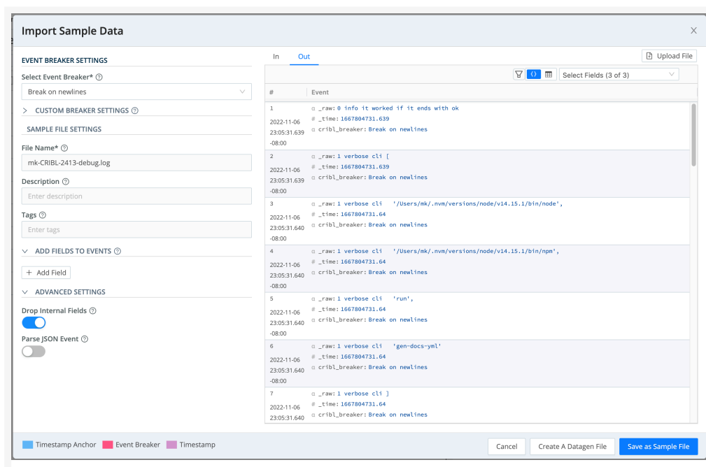
Example of imported data
