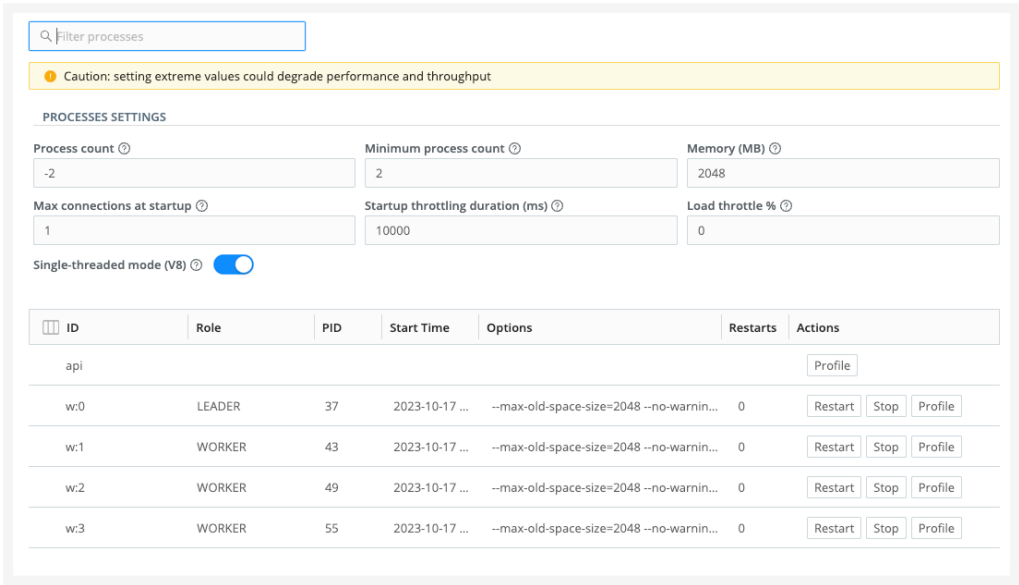
Worker CPU profiling (single-instance)
