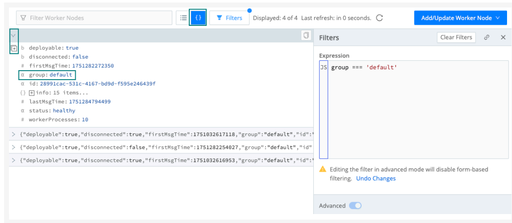
Filter Worker Nodes in JSON view
