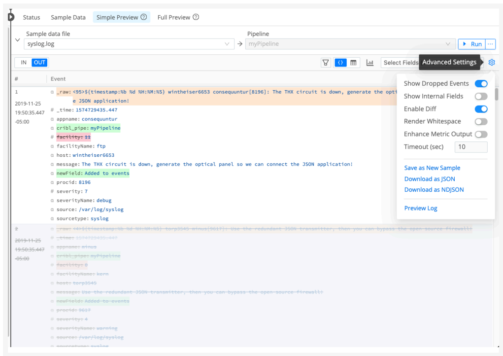
Highlighted fields in Pipeline output
