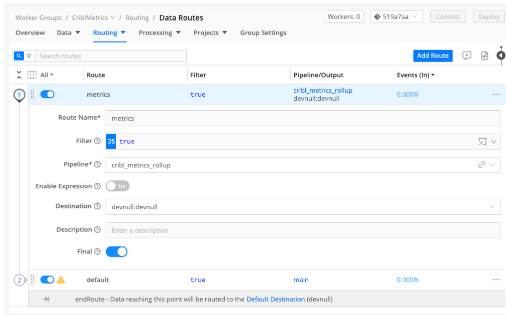
Cribl metrics Route, Pipeline, and Destination wired up
