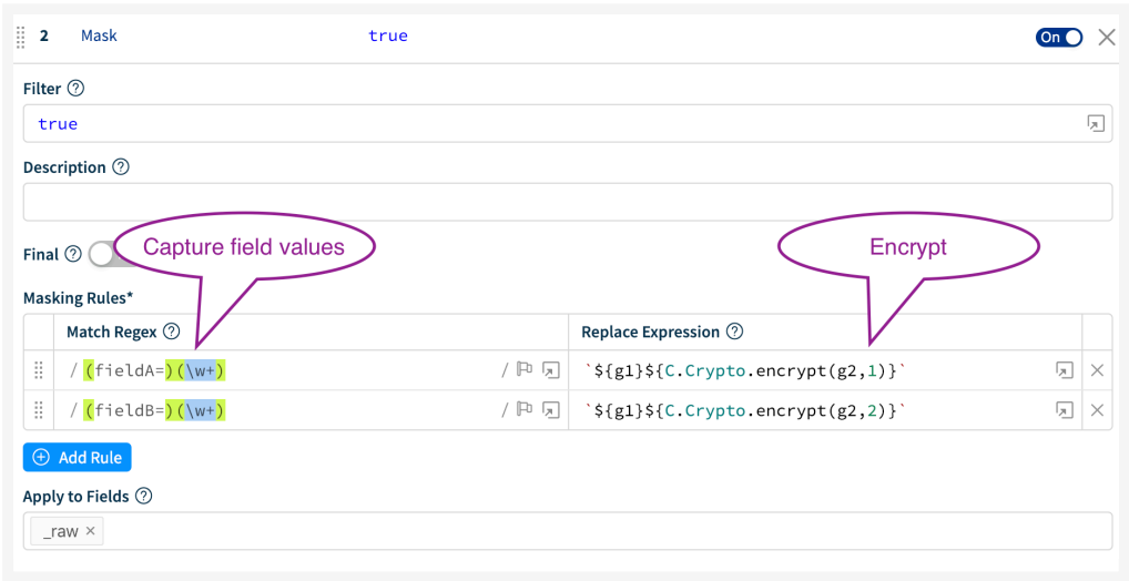
Encrypting two fields with separate key classes
