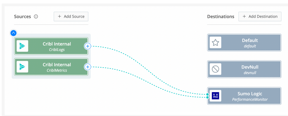
Cribl Internal forwarding to Sumo Logic
