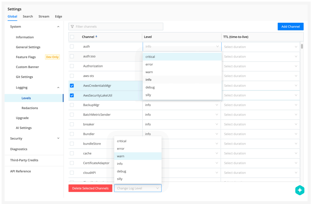
Levels page for managing logging levels
