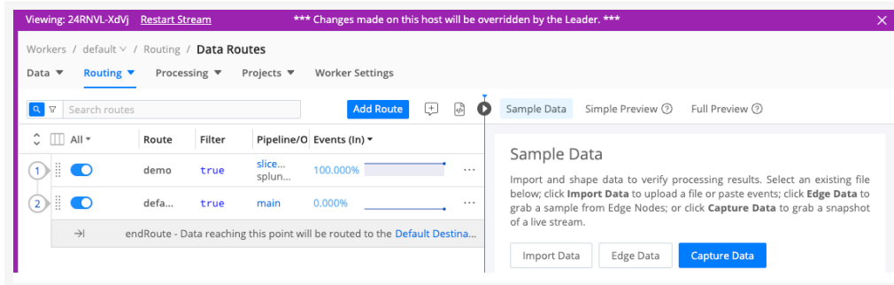
Leader's remote view of Worker's UI
