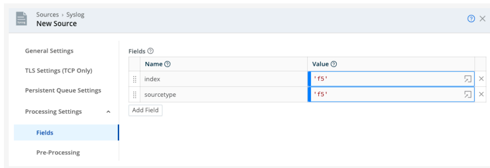
Metadata fields tied to a dedicated-port Syslog source
