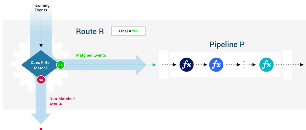
Data flow for a Route with Final toggled on
