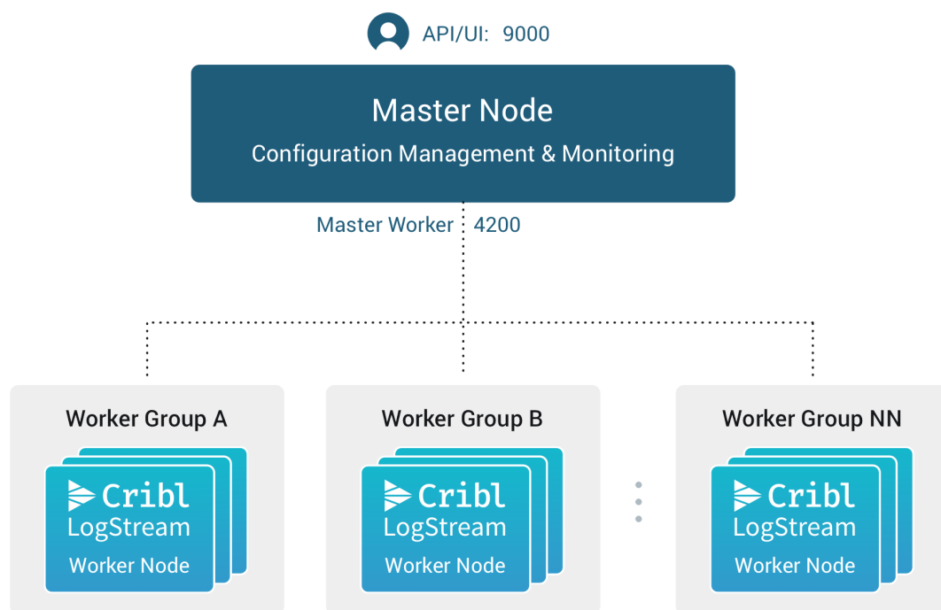
Master Node/Worker Nodes relationship
