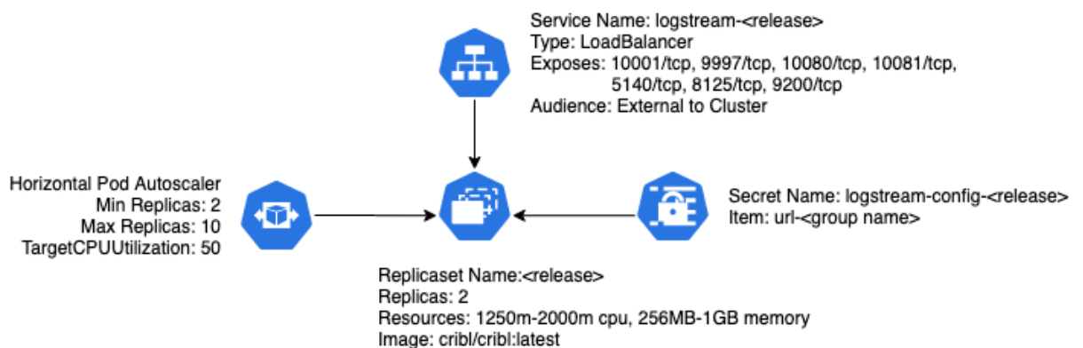
Deployment schematic
